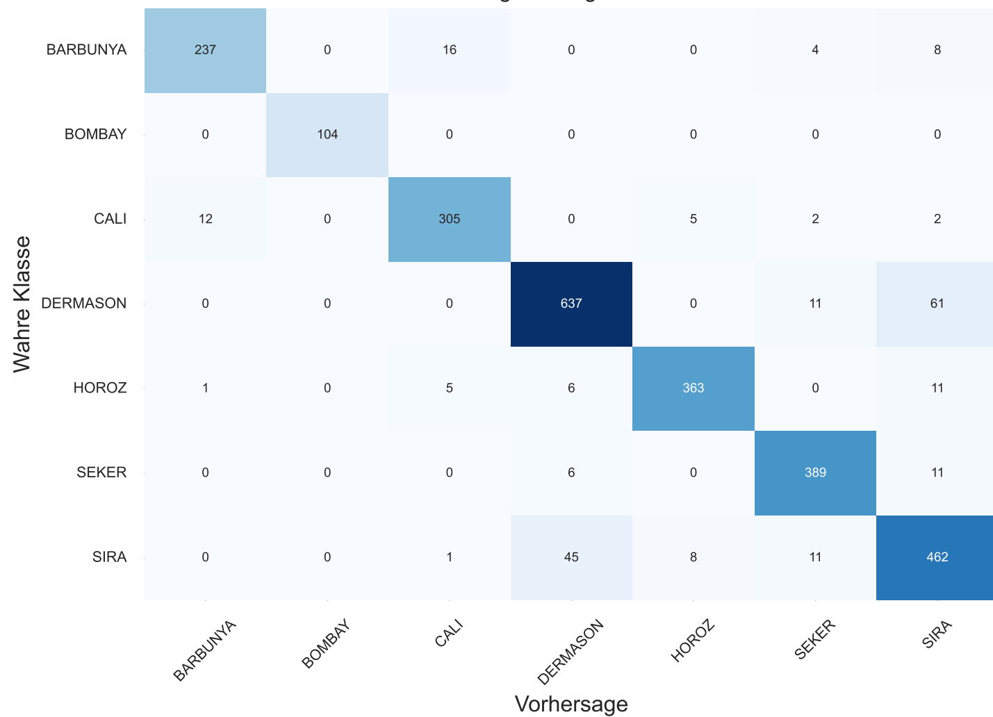
Logistic Regression
