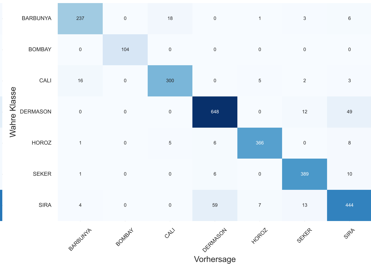
Random Forest
