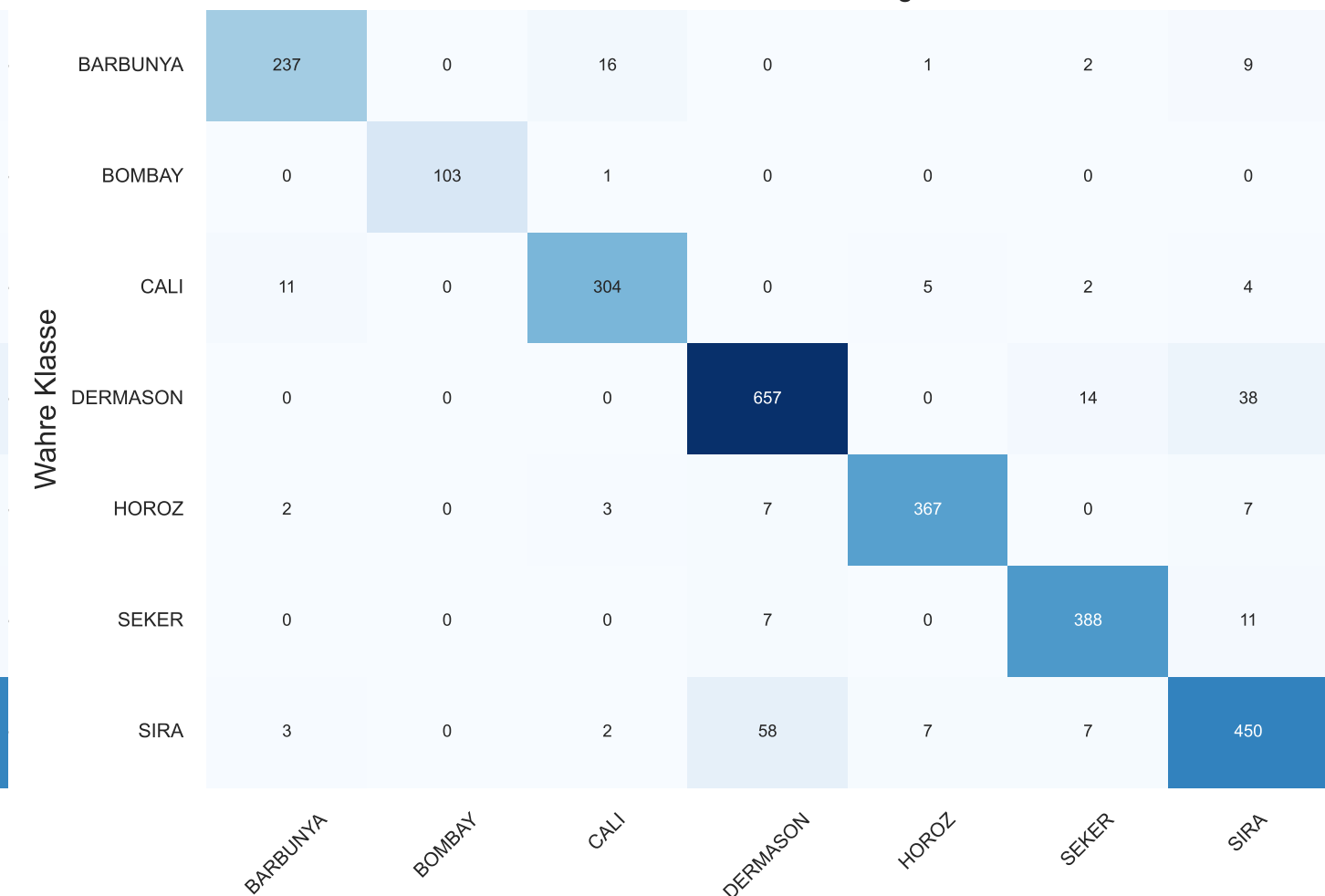
Hist Gradient Boosting
